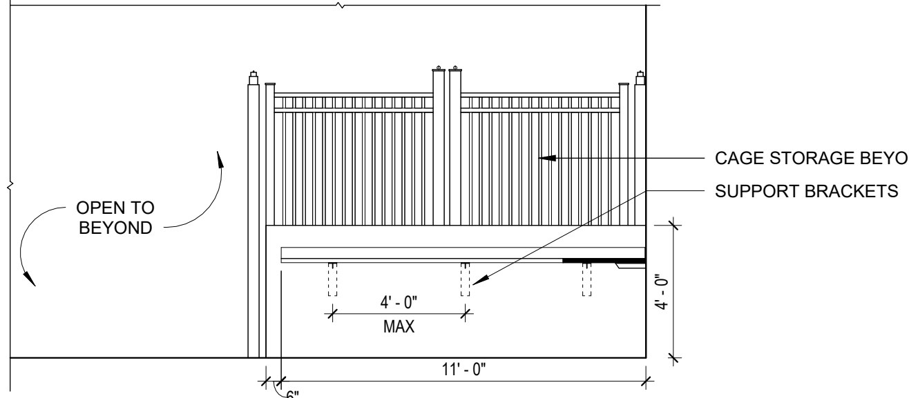
19 137 - N SHIPPING & RECEIVING 1/4" = 1'-0"
