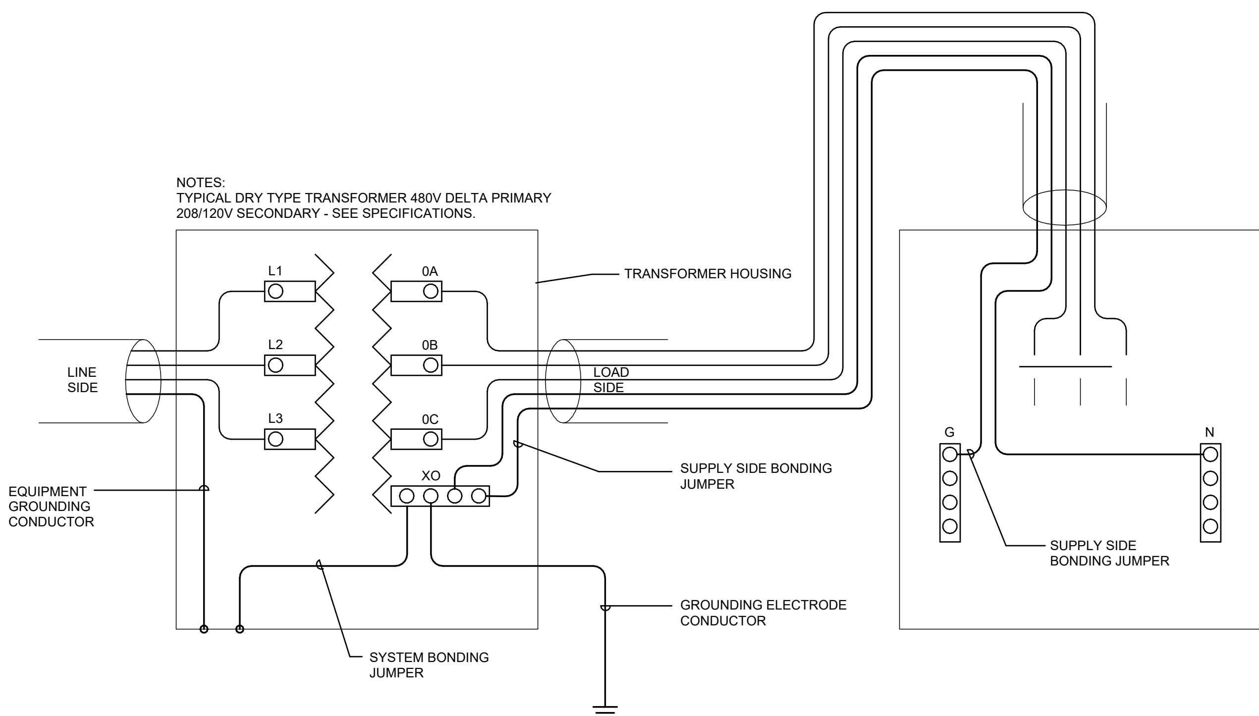
7 TRANSFORMER WIRING SCALE: NTS
