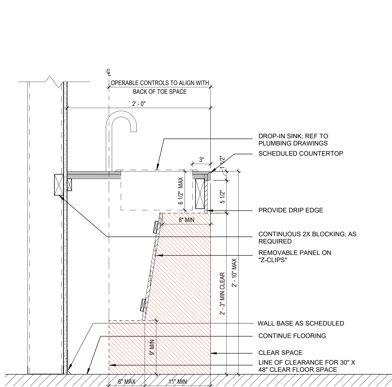
04 SECTION AT TAMBOUR PANEL 1 1/2" = 1'-0"
