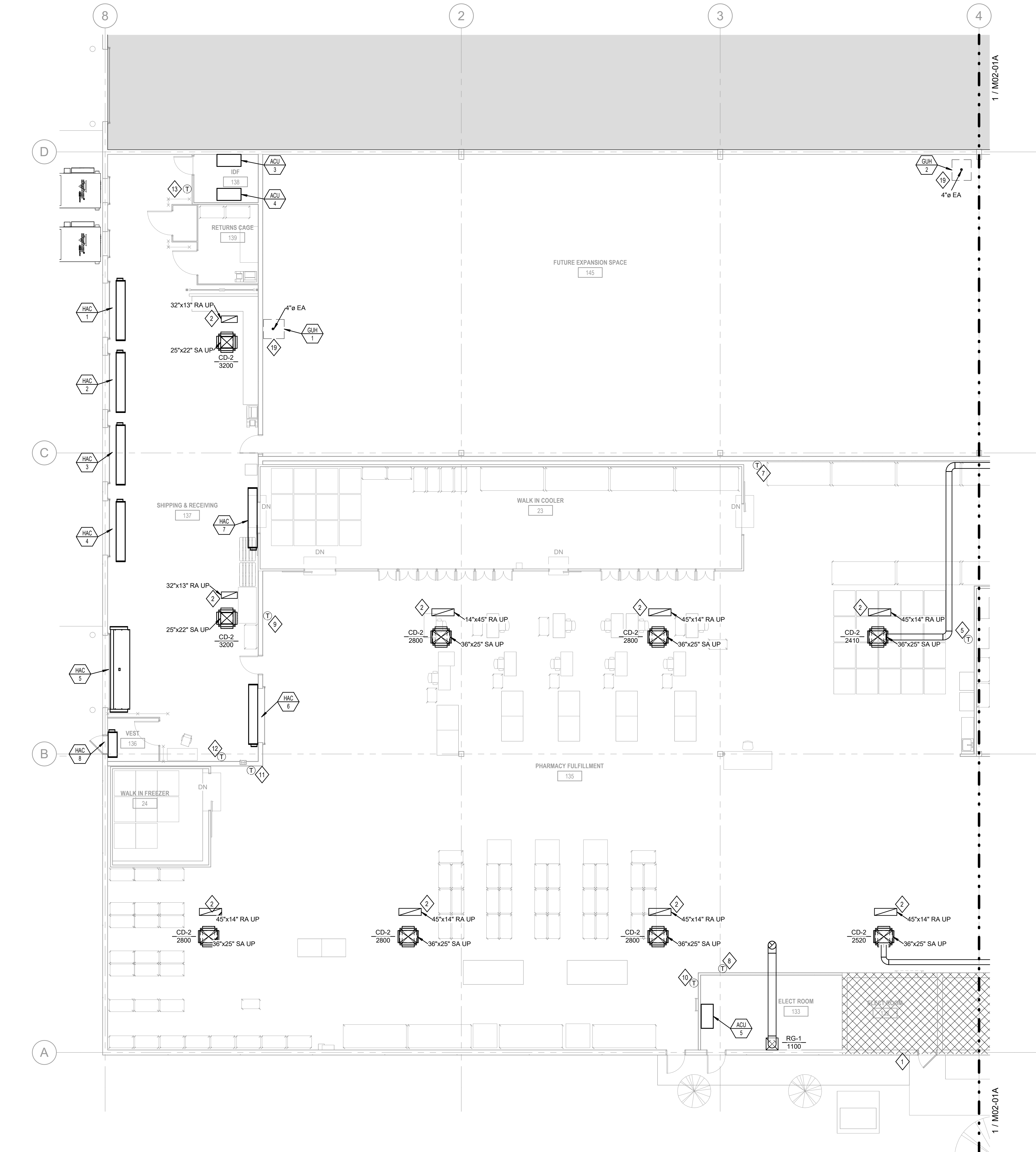
1 HVAC PLAN - LEVEL ONE - SEGMENT B SCALE: 1/8" = 1'-0"
