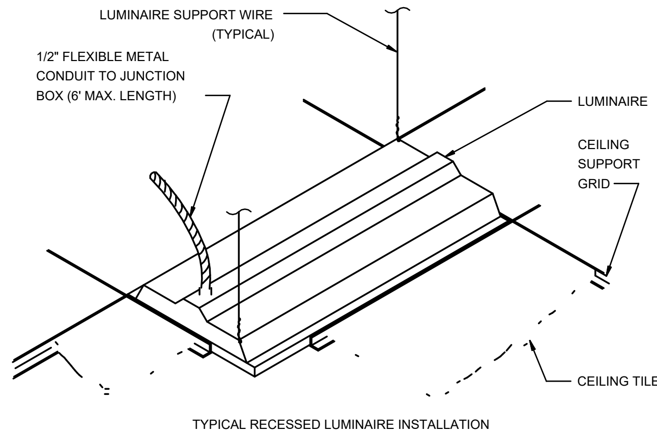
5 RECESSED LUMINAIRE SUPPORT SCALE: NTS
