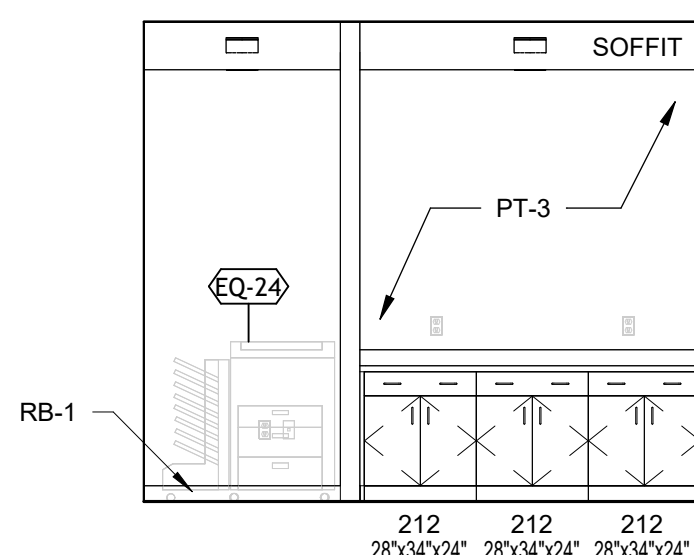
7 113 - W COPY 1/4" = 1'-0"
