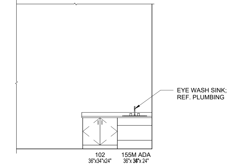
20 135 - S PHARMACY FULFILLMENT 1/4" = 1'-0"
