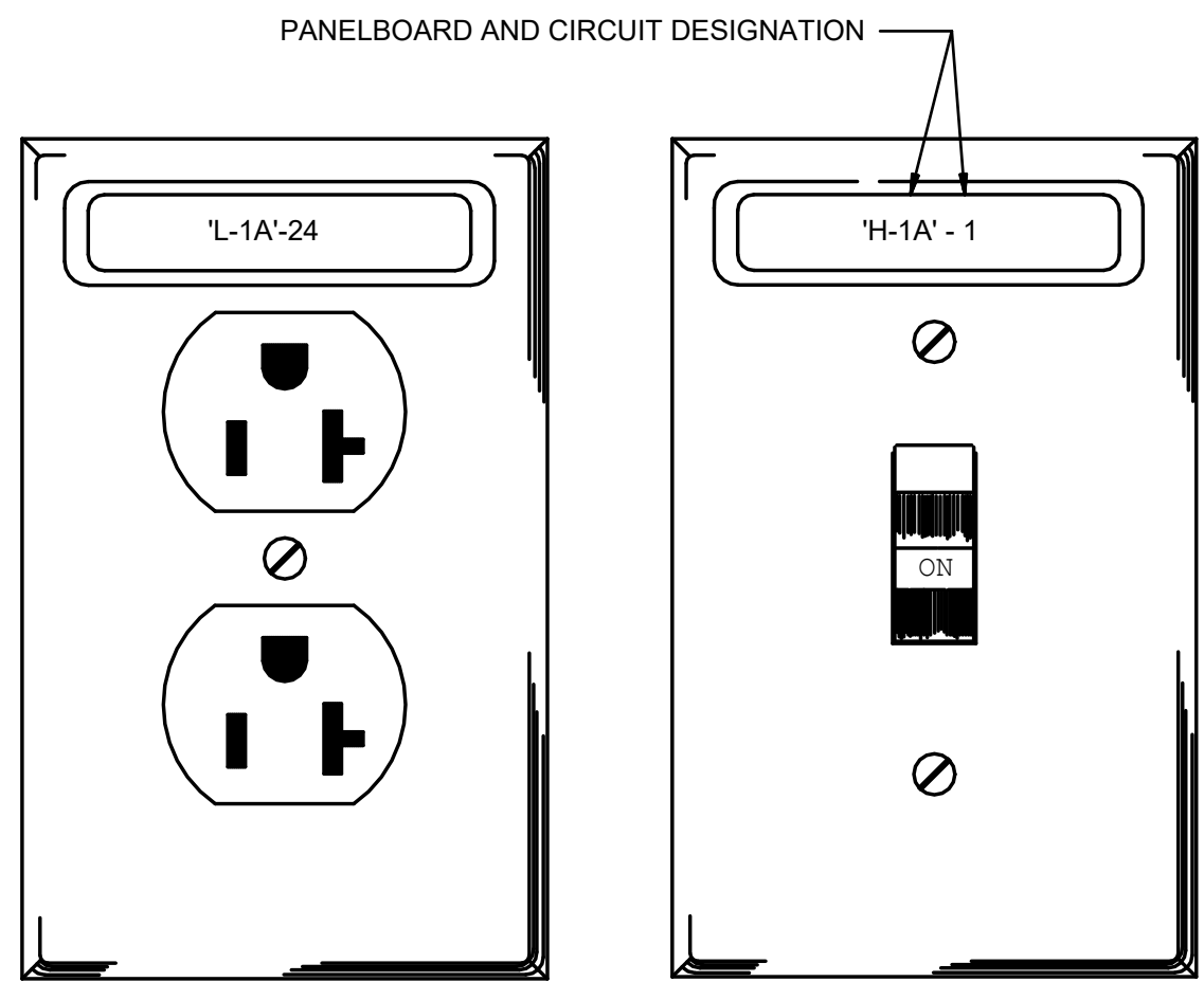
4 RECEPTACLE/SWITCH IDENTIFICATION SCALE: NTS
