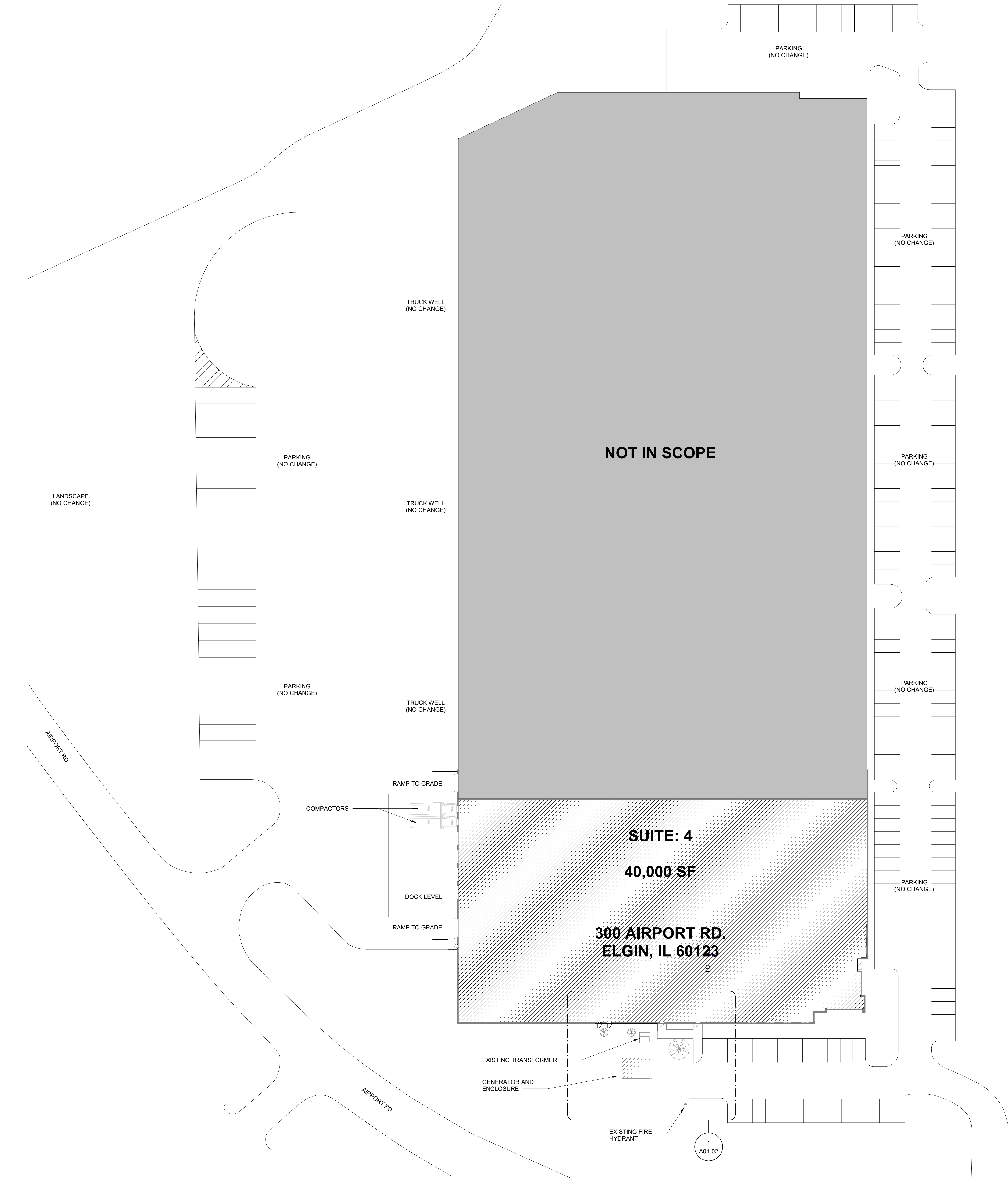
1 SITE PLAN 1" = 30'-0"
