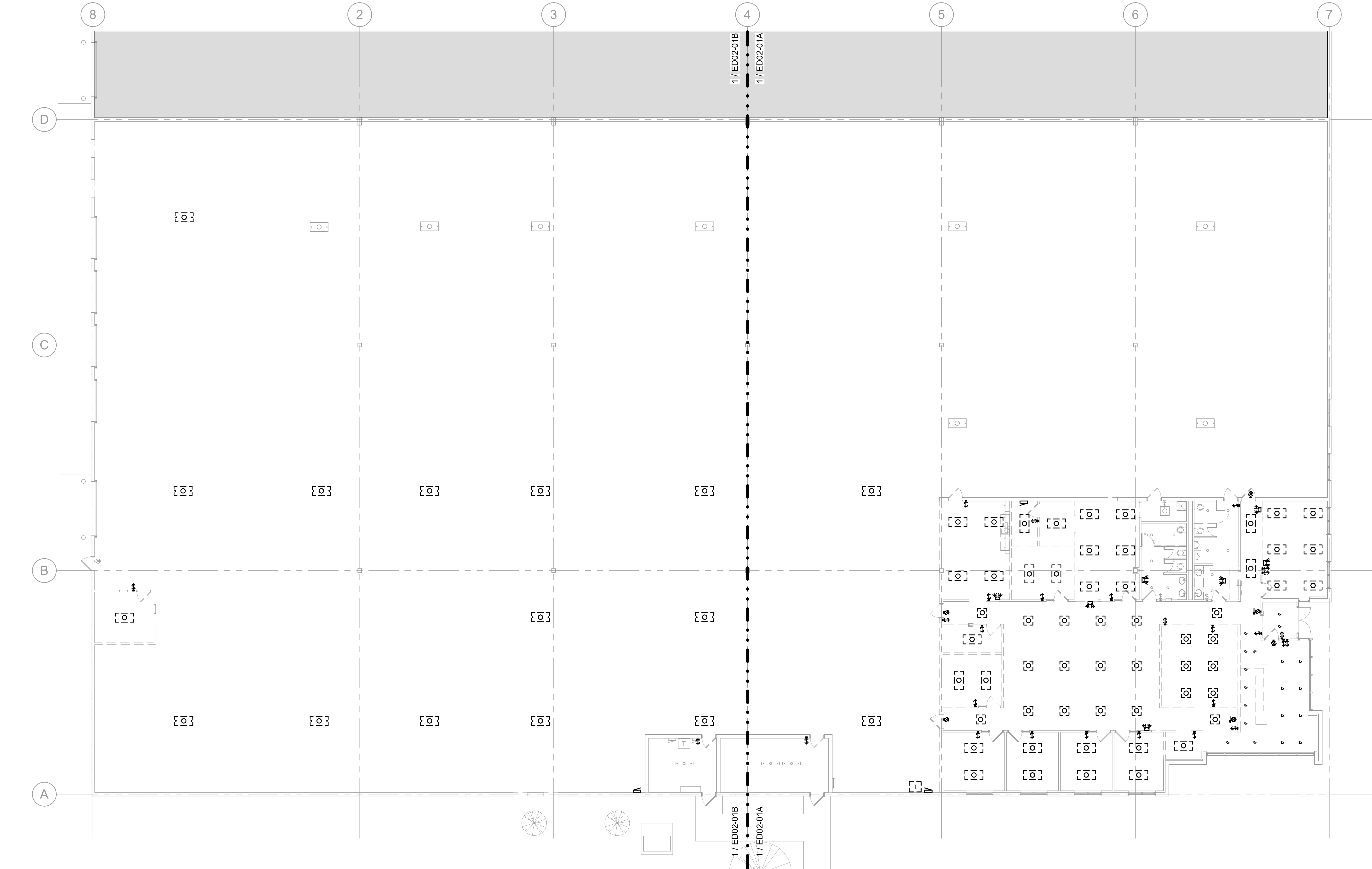
1 LIGHTING DEMOLITION PLAN - LEVEL ONE SCALE: 3/32" = 1'-0"
