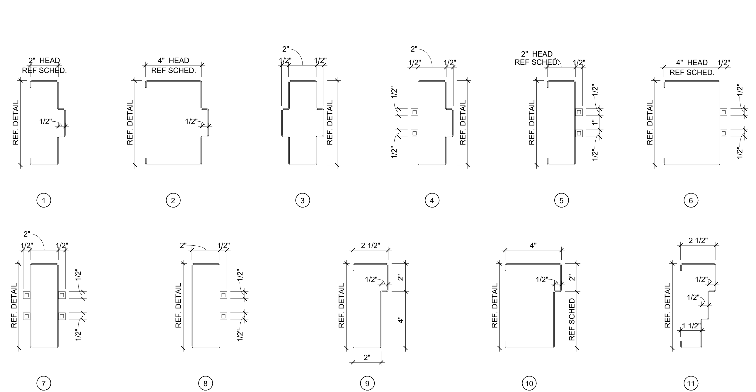
H.M. FRAME PROFILES 3" = 1'-0"
