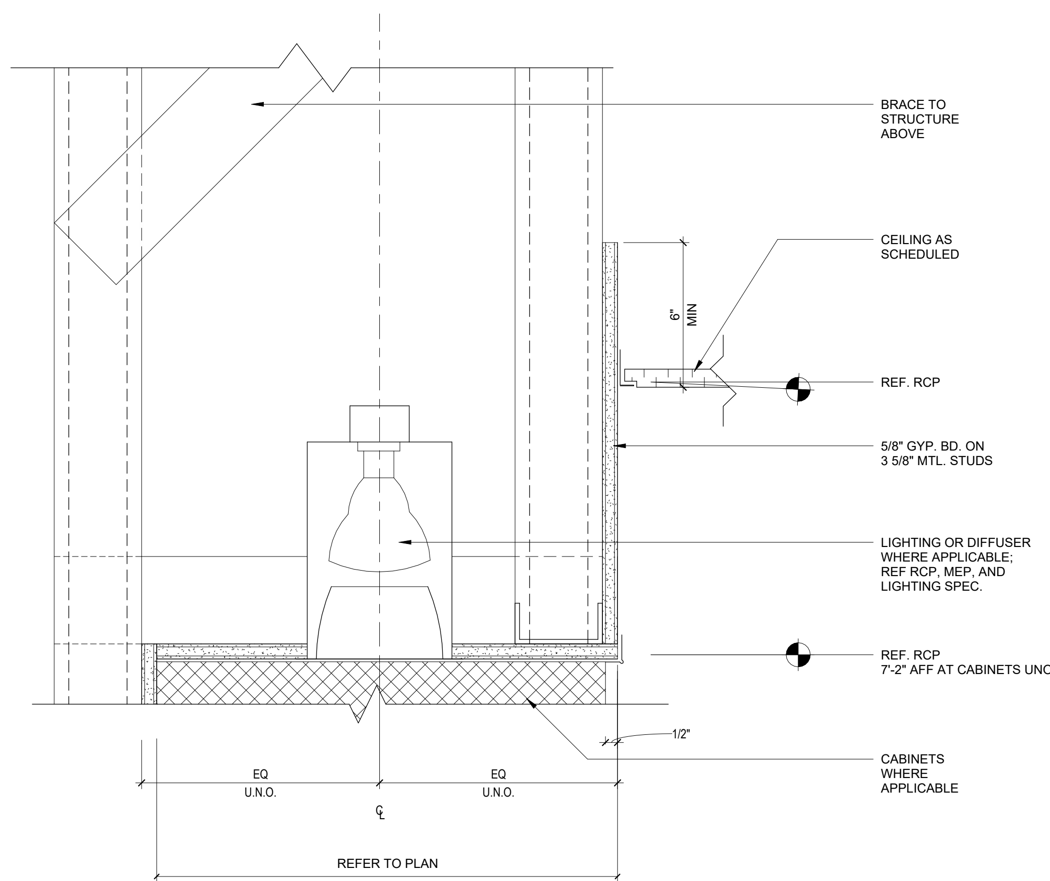
4 SECTION AT TYPICAL TV NICHE 1 1/2" = 1'-0"
