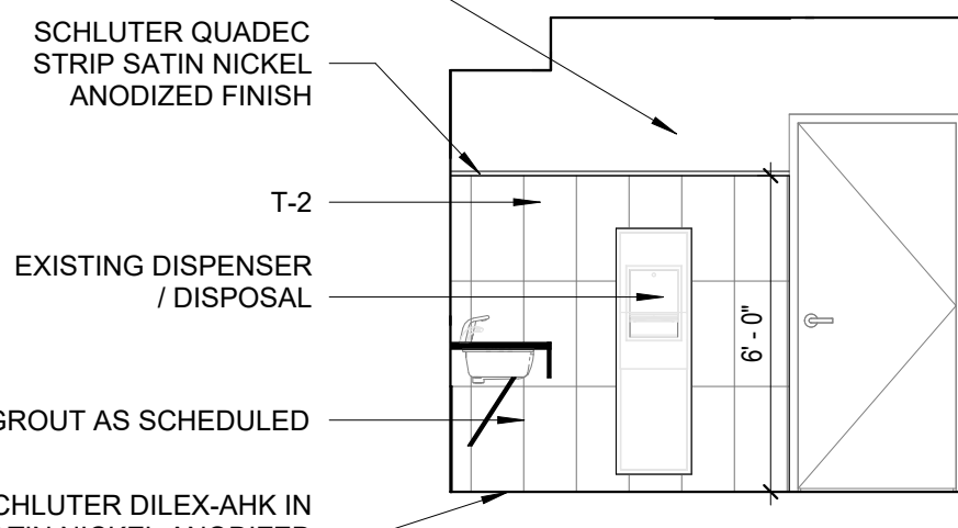
3 124 - WOMENS RR S 1/4" = 1'-0"
