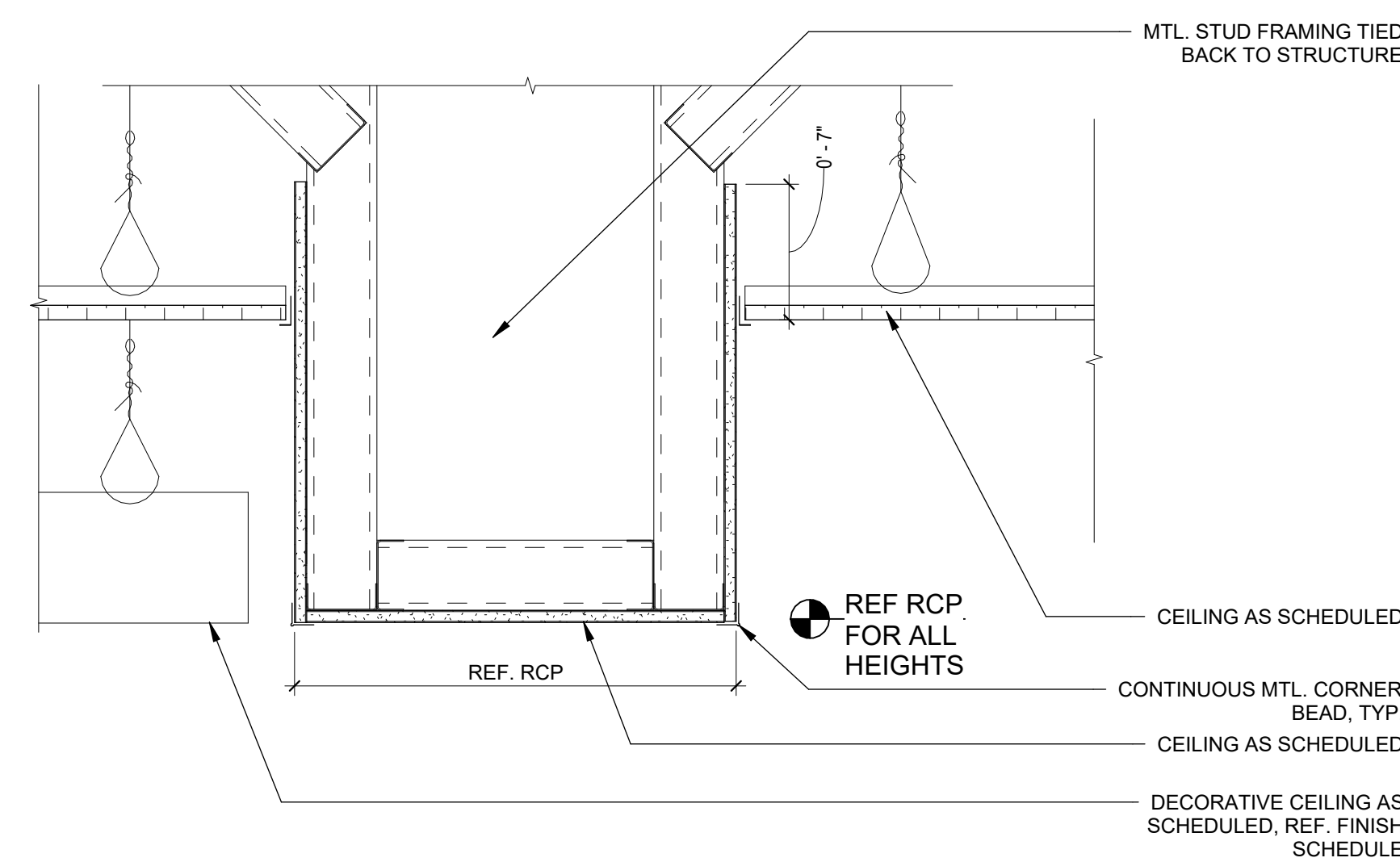
5 RCP DETAIL - GYP HEADER DECORATIVE CEILING 1 1/2" = 1'-0"
