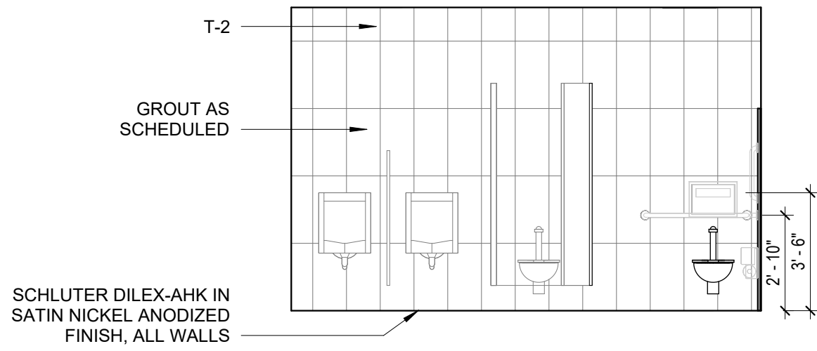
8 125 - MENS RR STALLS W 1/4" = 1'-0"
