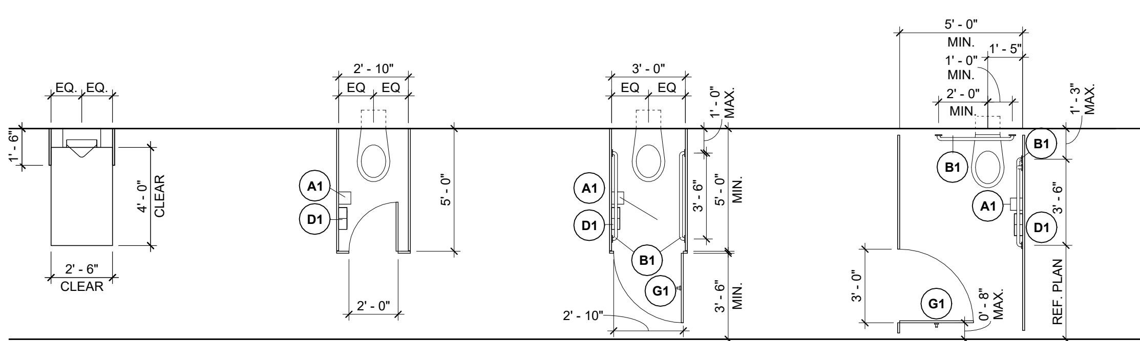
STALL TYPES DIAGRAMS
