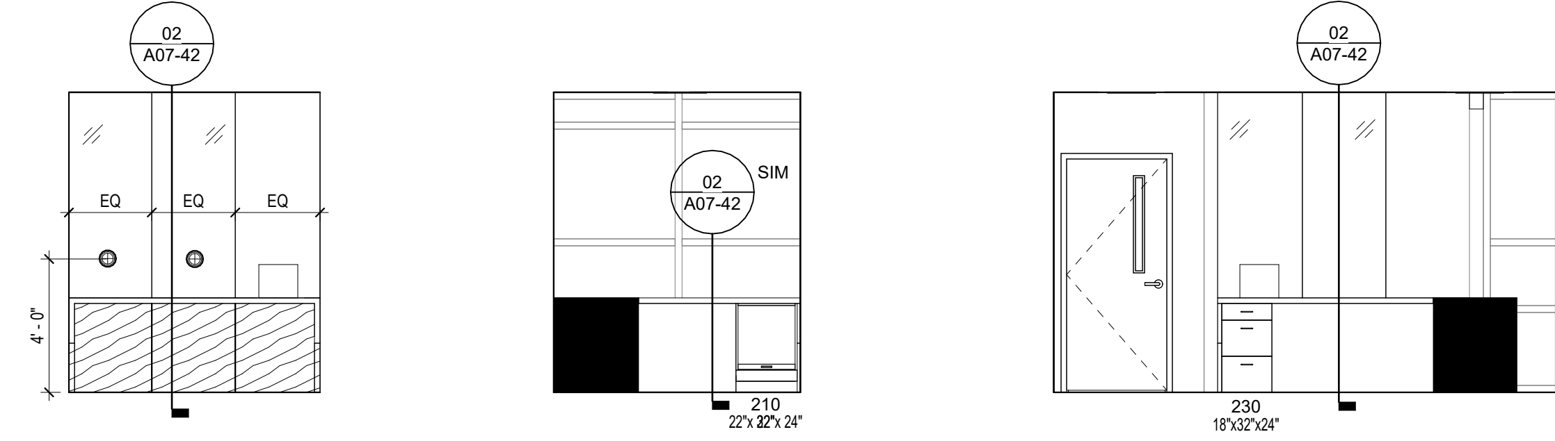
16 103 - S SECURITY/RECEPTION 1/4" = 1'-0"
