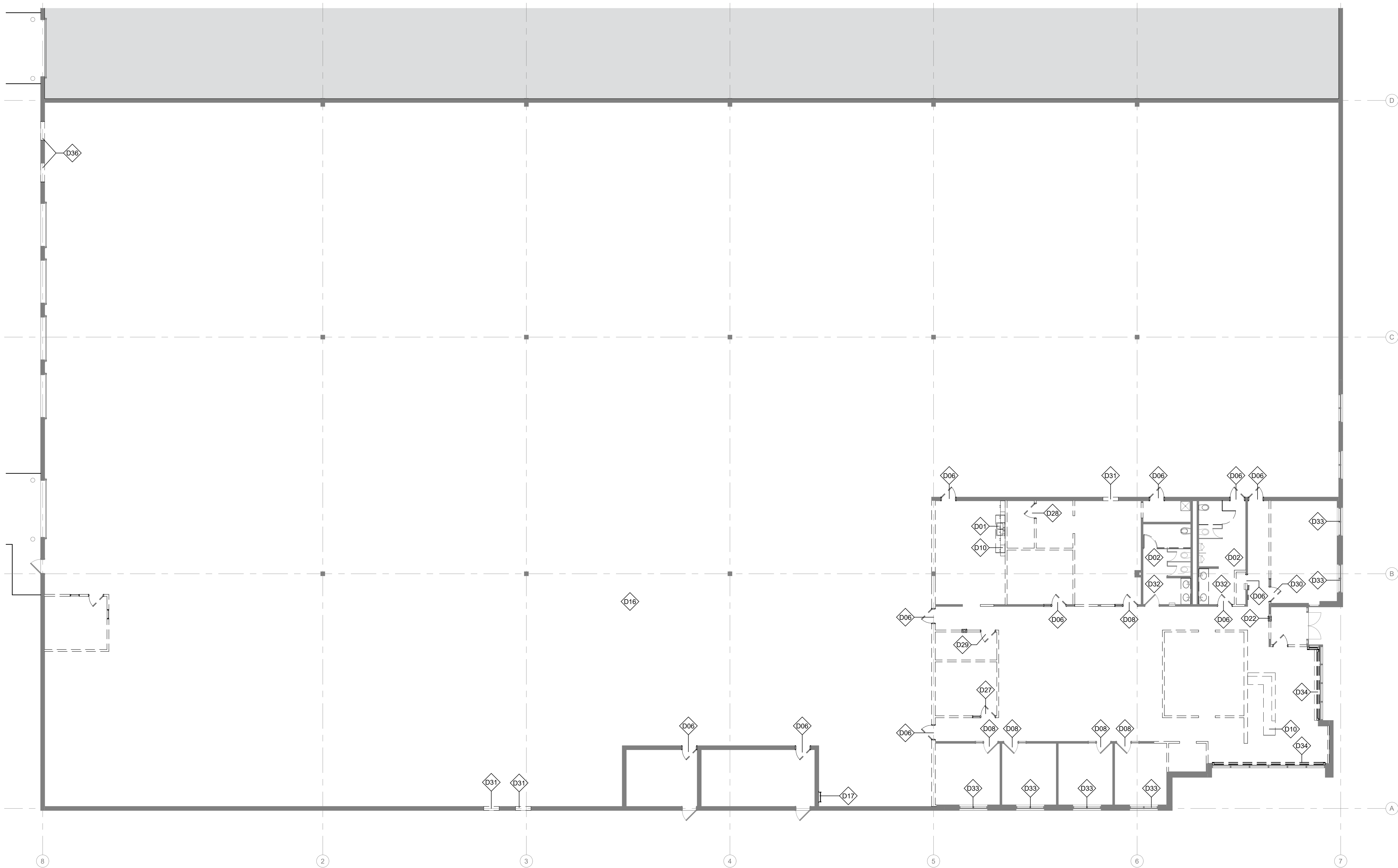
1 DEMO FLOOR PLAN - OVERALL 3/32" = 1'-0"
