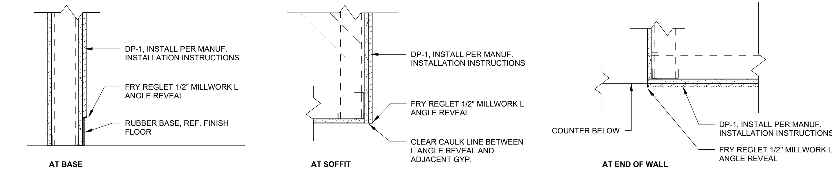
04 SECTION AT TAMBOUR PANEL 1 1/2" = 1'-0"
