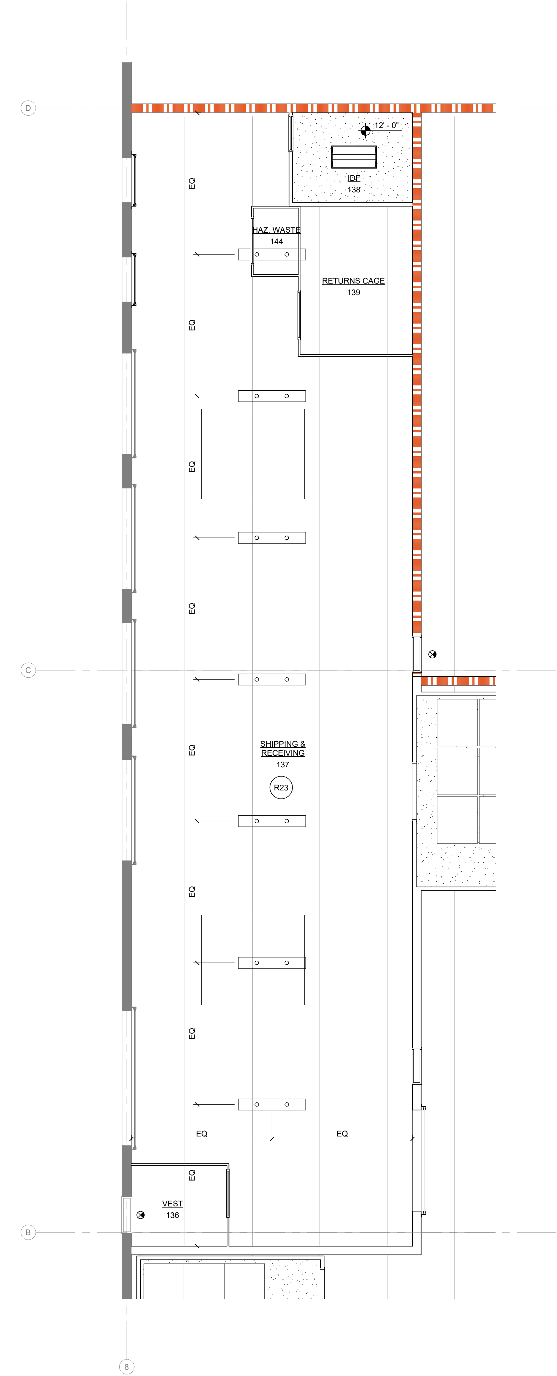
1 REFLECTED CEILING PLAN - SEGMENT B 3/16" = 1'-0"
