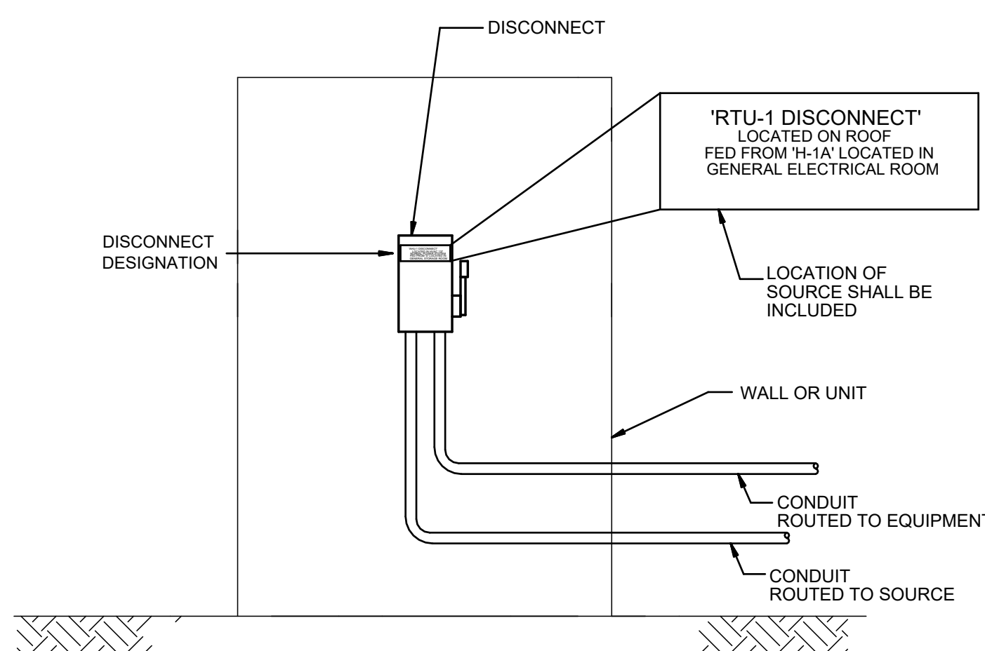
3 DISCONNECT IDENTIFICATION SCALE: NTS
