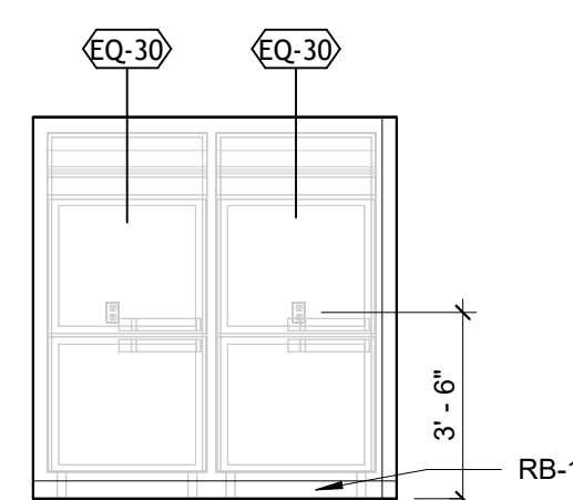
2 104 - S BREAKROOM 1/4" = 1'-0"
