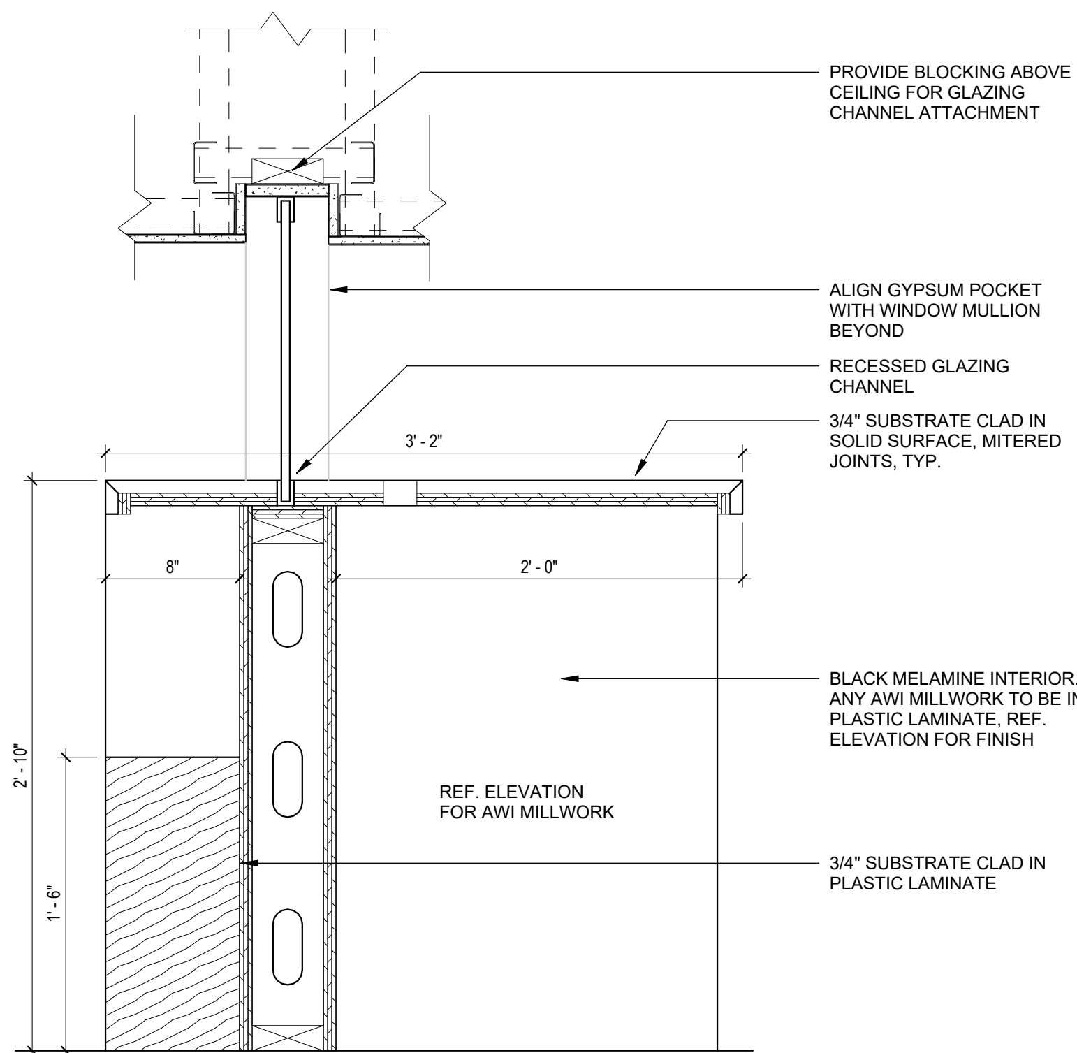
02 SECTION AT RECEPTION TRANSACTION 1 1/2" = 1'-0"
