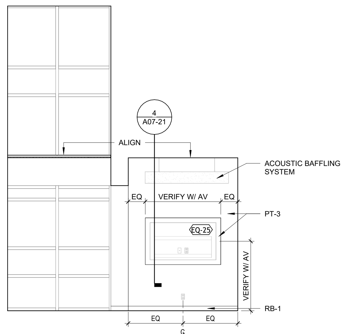
1 104 - E BREAKROOM 1/4" = 1'-0"
