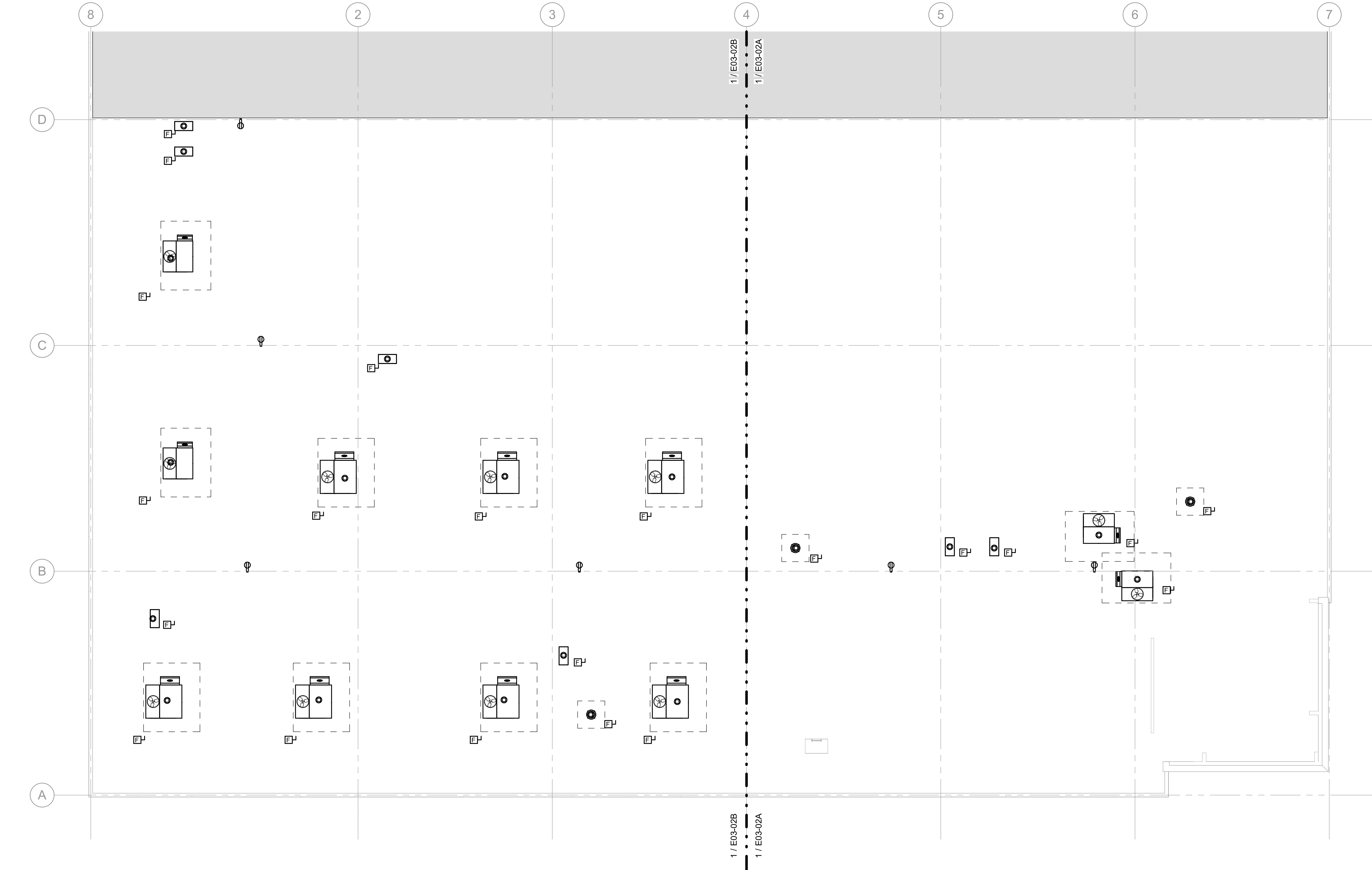
1 POWER PLAN - ROOF SCALE: 3/32" = 1'-0"
