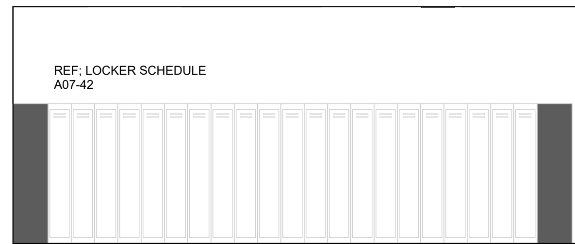
11 116 - N LOCKERS 1/4" = 1'-0"
