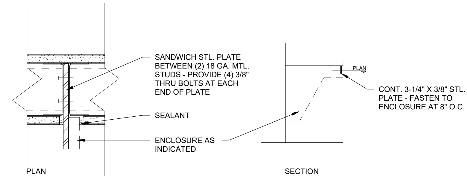
02 LAVATORY COUNTER SUPPORT - SPAN LESS THAN 10'-0" N.T.S.
