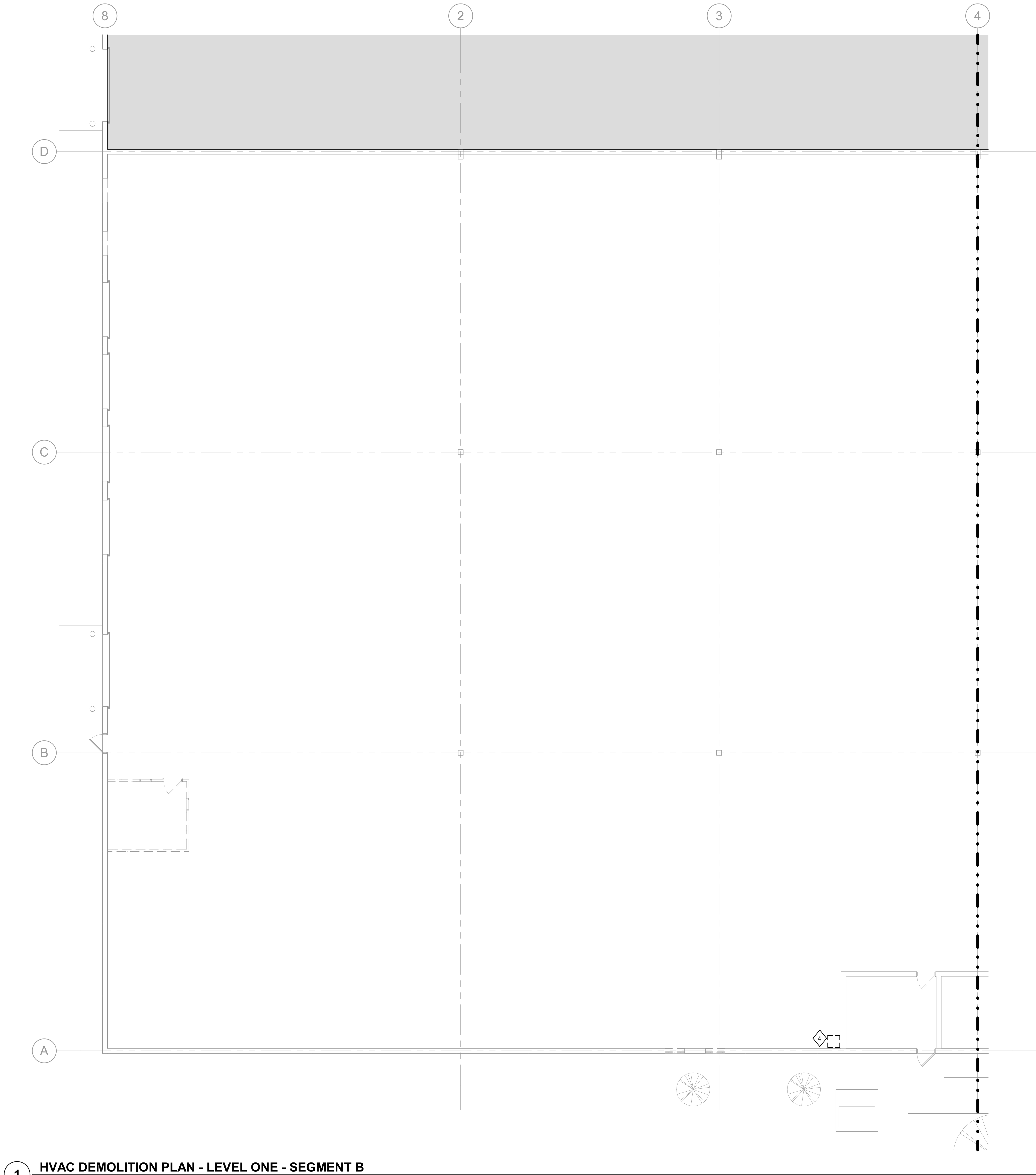
1 HVAC DEMOLITION PLAN - LEVEL ONE - SEGMENT B SCALE: 1/8" = 1'-0"
