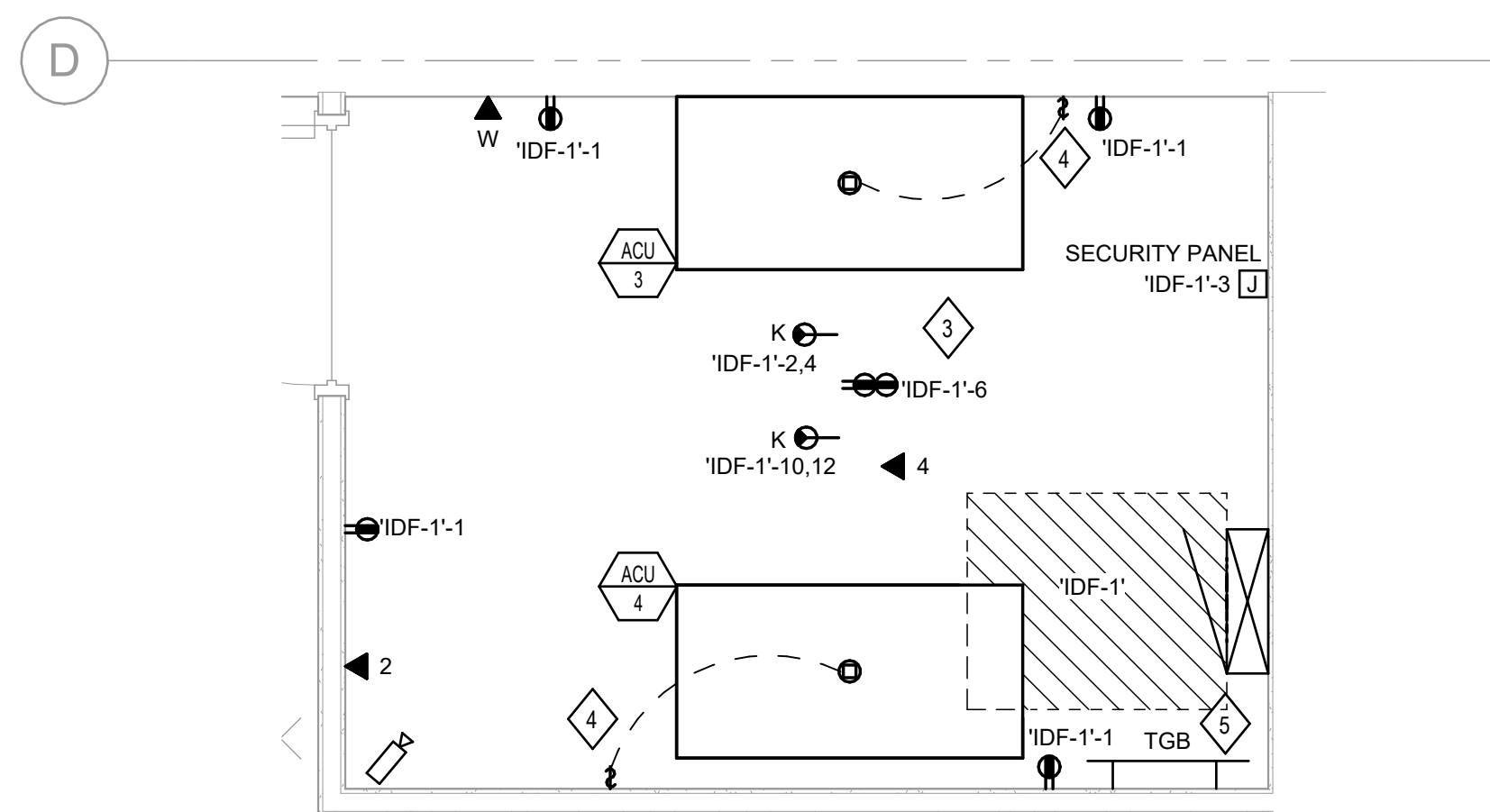
2 POWER PLAN - LEVEL ONE - SEGMENT B - SHIPPING & RECEIVING IDF SCALE: 1/2" = 1'-0"
