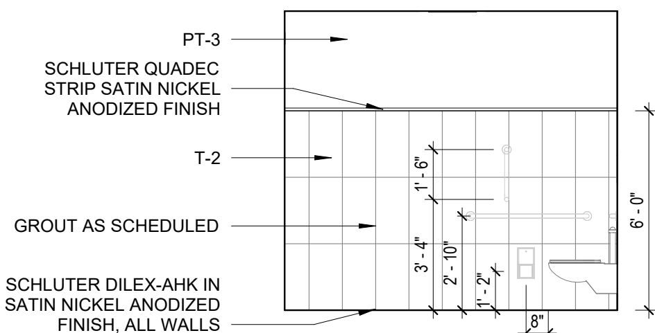
4 124 - WOMENS RR TLT N 1/4" = 1'-0"
