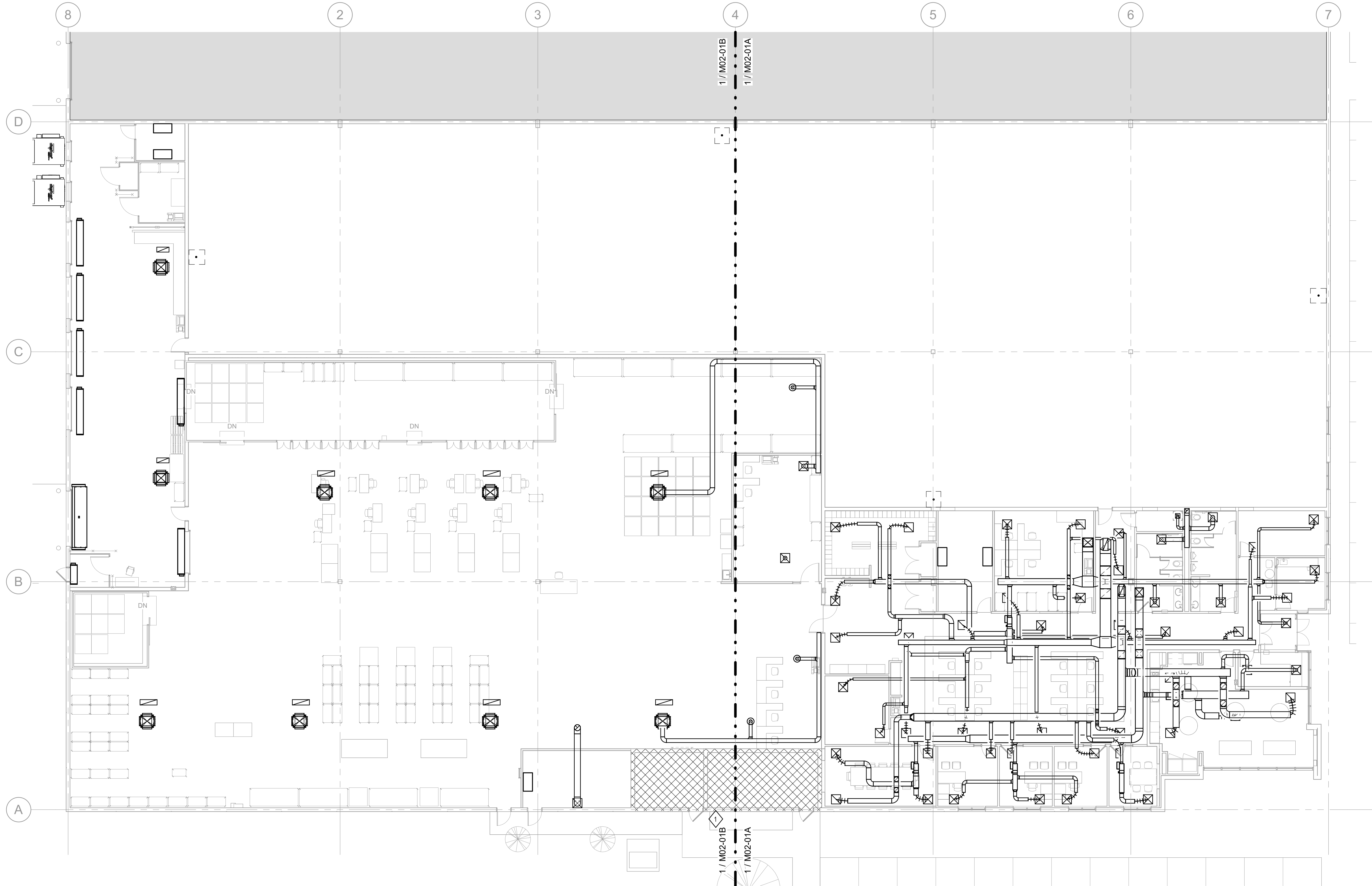
1 HVAC PLAN - LEVEL ONE SCALE: 3/32" = 1'-0"
