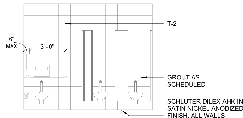
5 124 - WOMENS RR STALLS E 1/4" = 1'-0"
