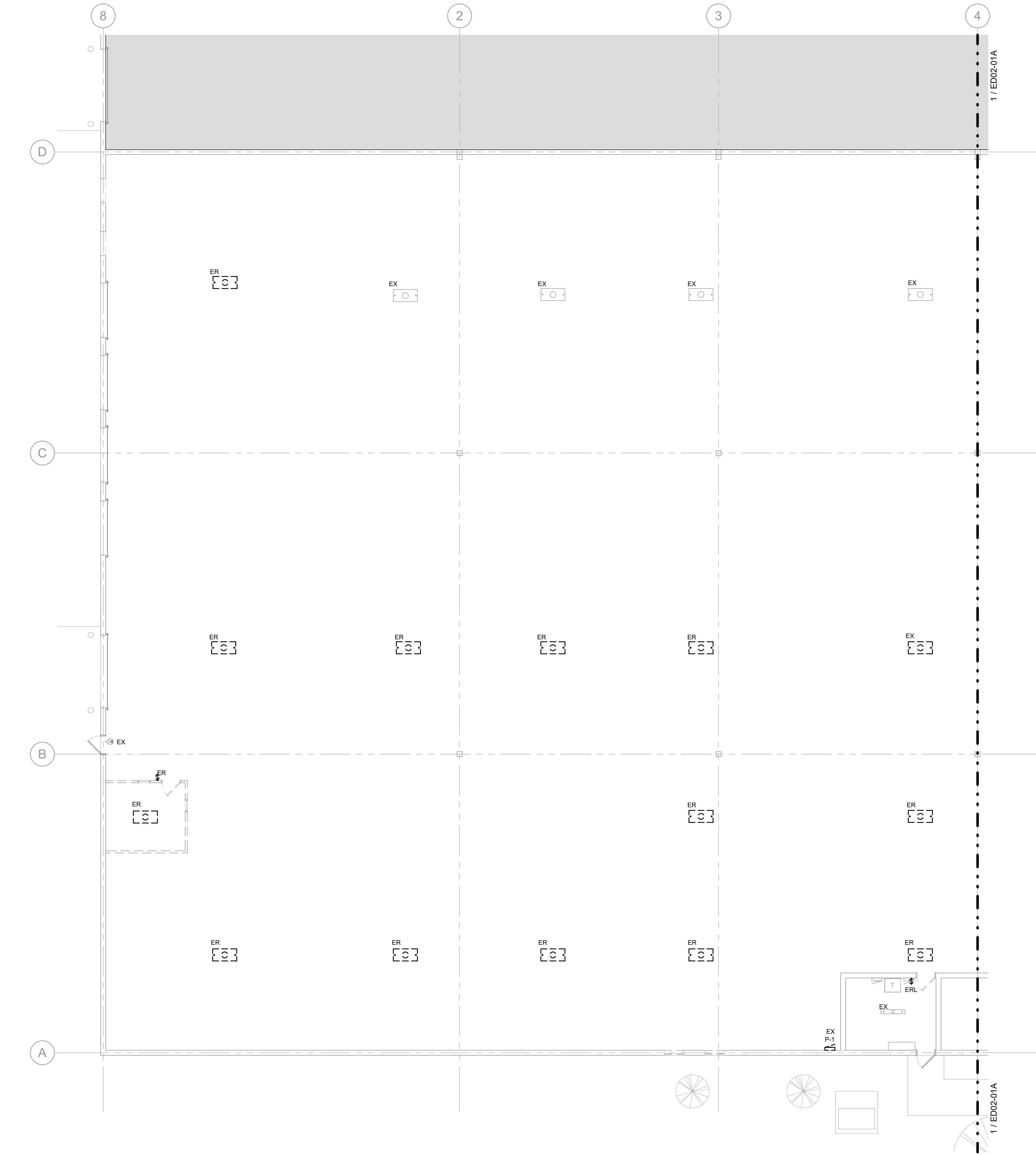
1 LIGHTING DEMOLITION PLAN - LEVEL ONE - SEGMENT B SCALE: 1/8" = 1'-0"
