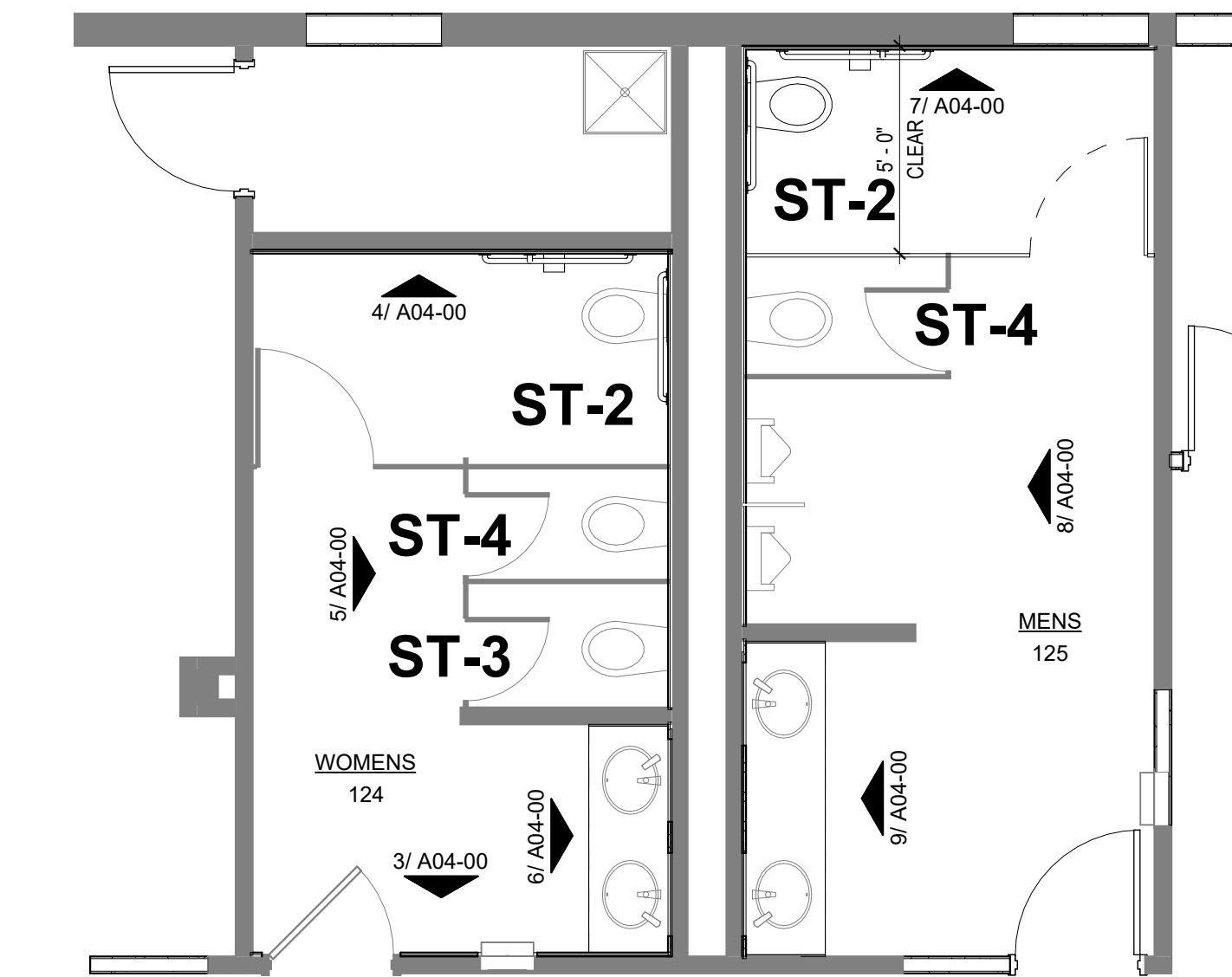
1 ENLARGED PLAN - RESTROOMS 1/4" = 1'-0"
