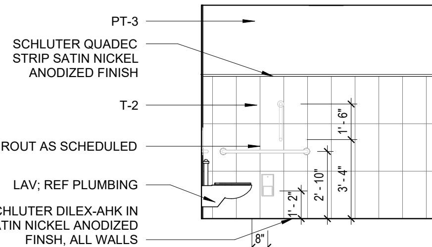
7 125 - MENS RR TLT N 1/4" = 1'-0"
