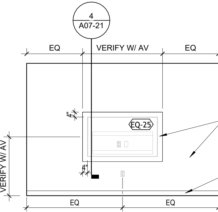
6 106 - E HUDDLE 1/4" = 1'-0"
