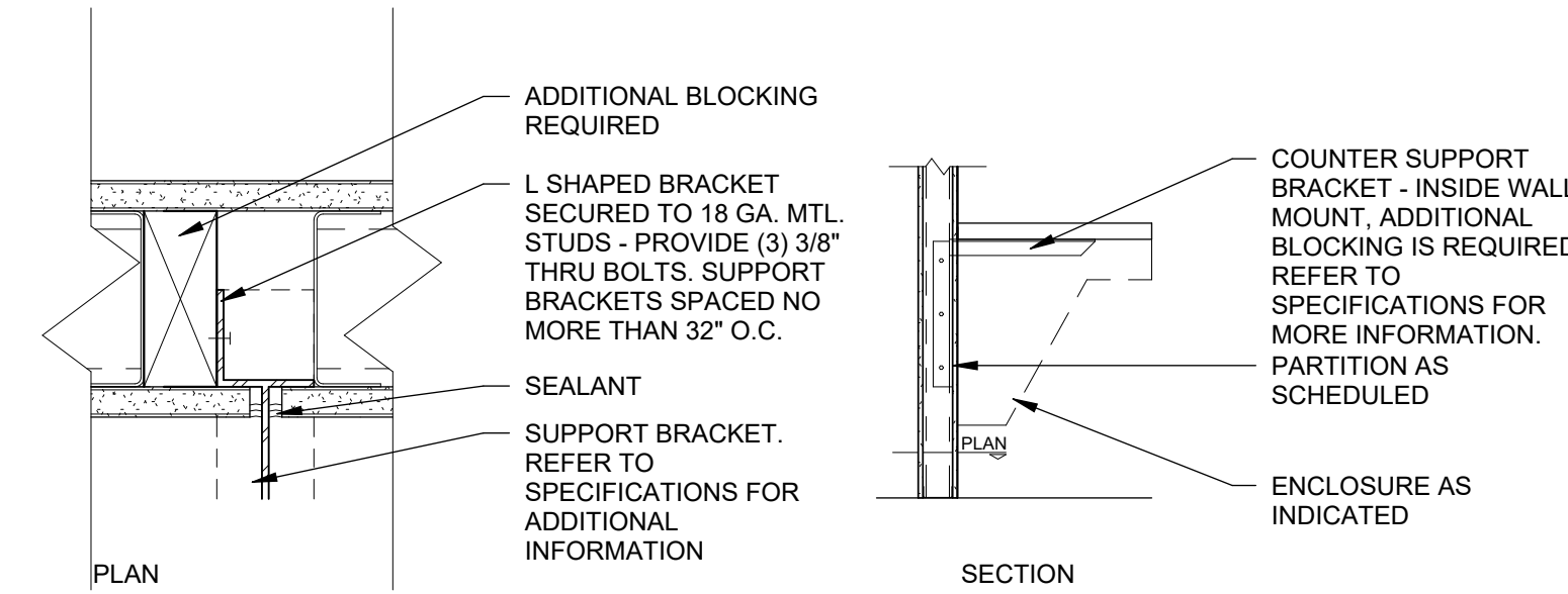
04 LAVATORY COUNTER SUPPORT BRACKETS - SPAN 10'-0" TO 16'-0" - SECTION N.T.S.
