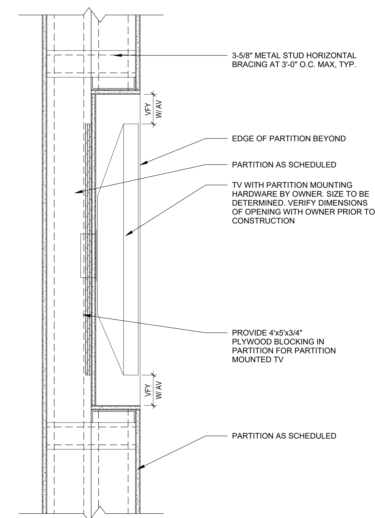
4 SECTION AT TYPICAL TV NICHE 1 1/2" = 1'-0"
