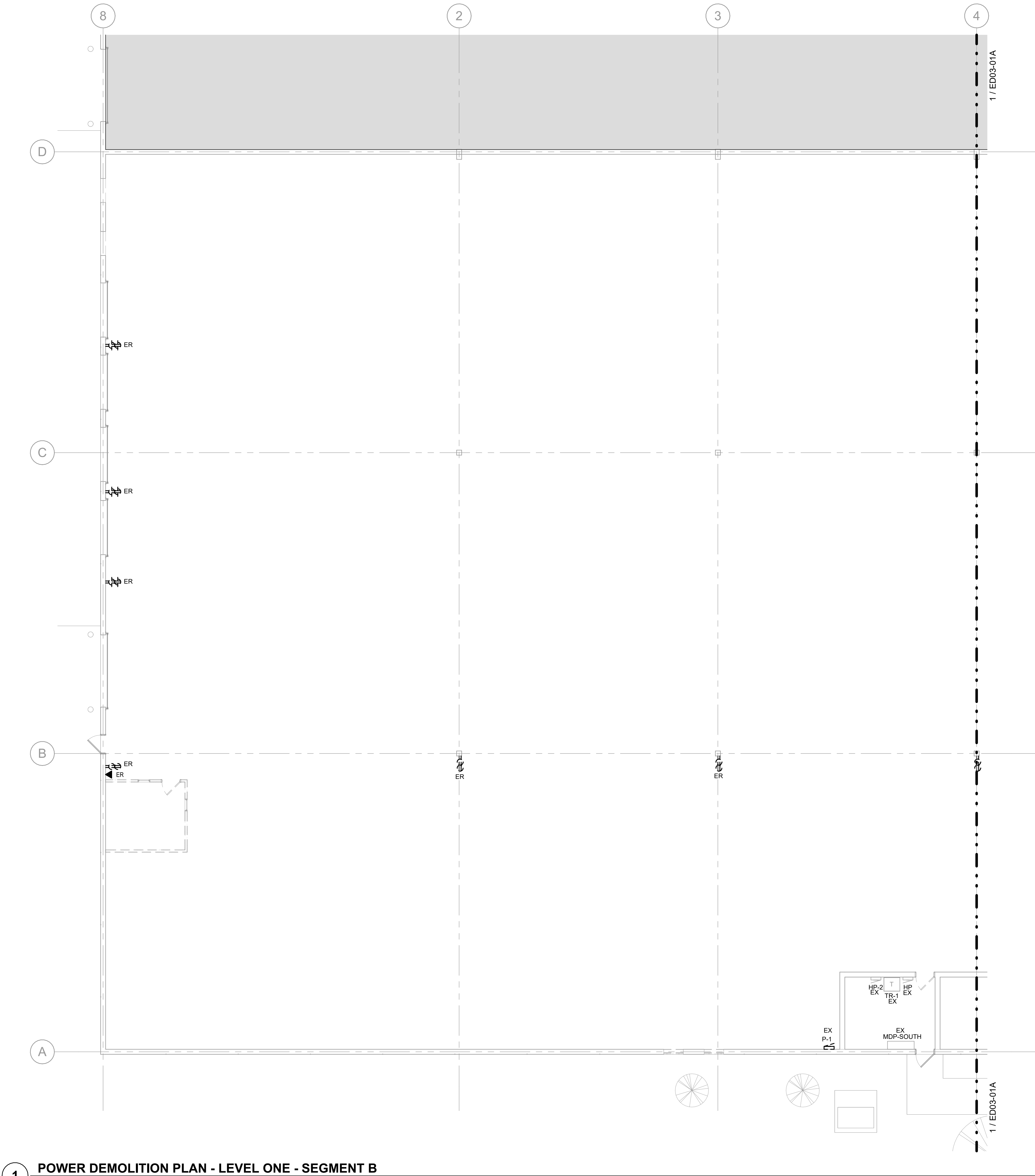
1 POWER DEMOLITION PLAN - LEVEL ONE - SEGMENT B SCALE: 1/8" = 1'-0"
