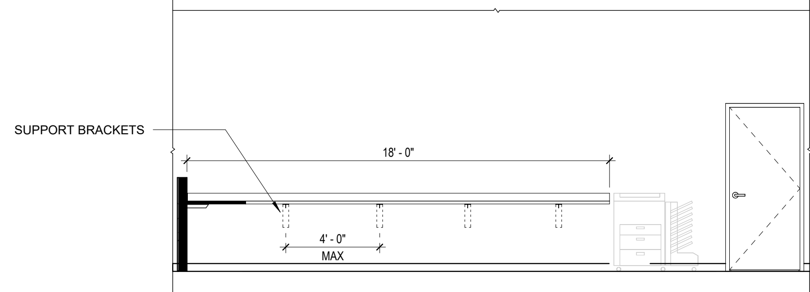
17 137 - E SHIPPING & RECEIVING 1/4" = 1'-0"
