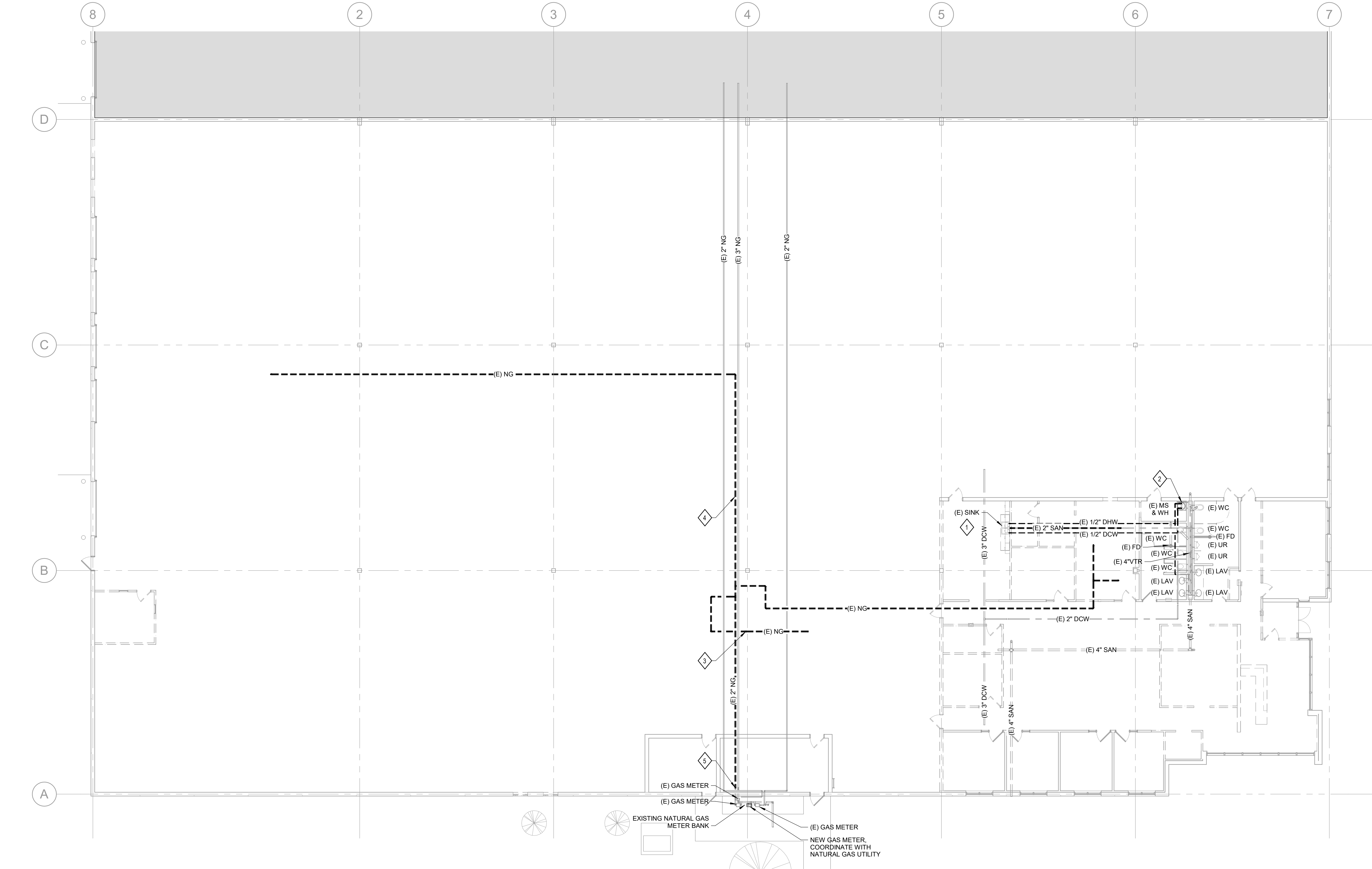
1 PLUMBING DEMOLITION PLAN - LEVEL ONE SCALE: 3/32" = 1'-0"
