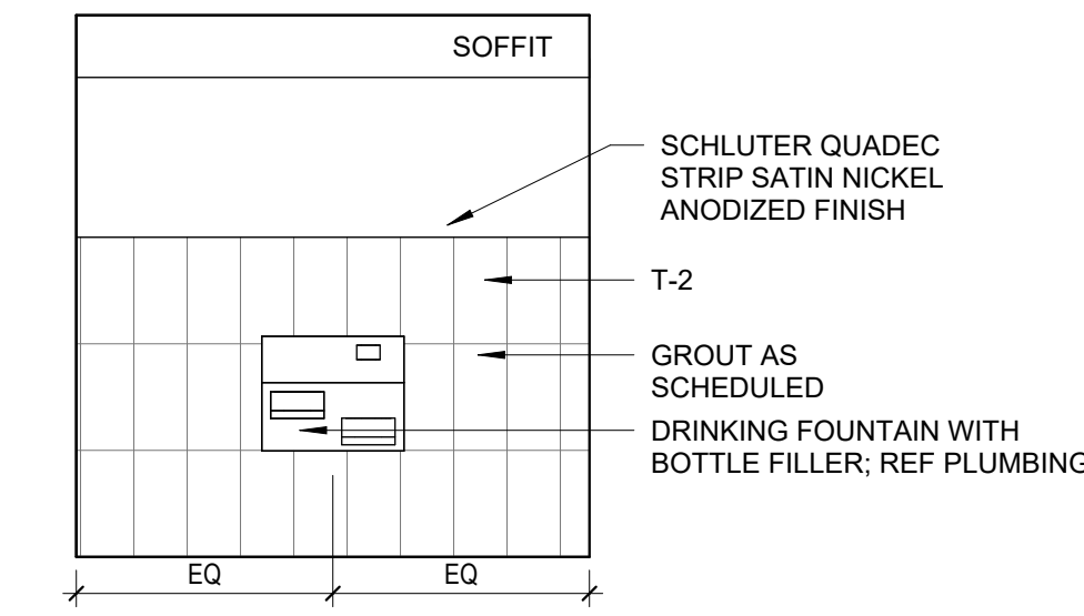
8 105 N DRINKING FOUNTAINS 1/4" = 1'-0"
