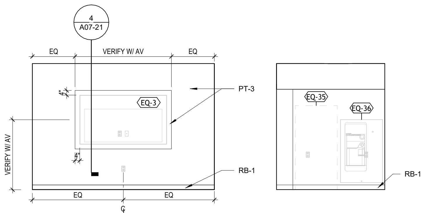
5 110 - W CONFERENCE 1/4" = 1'-0"
