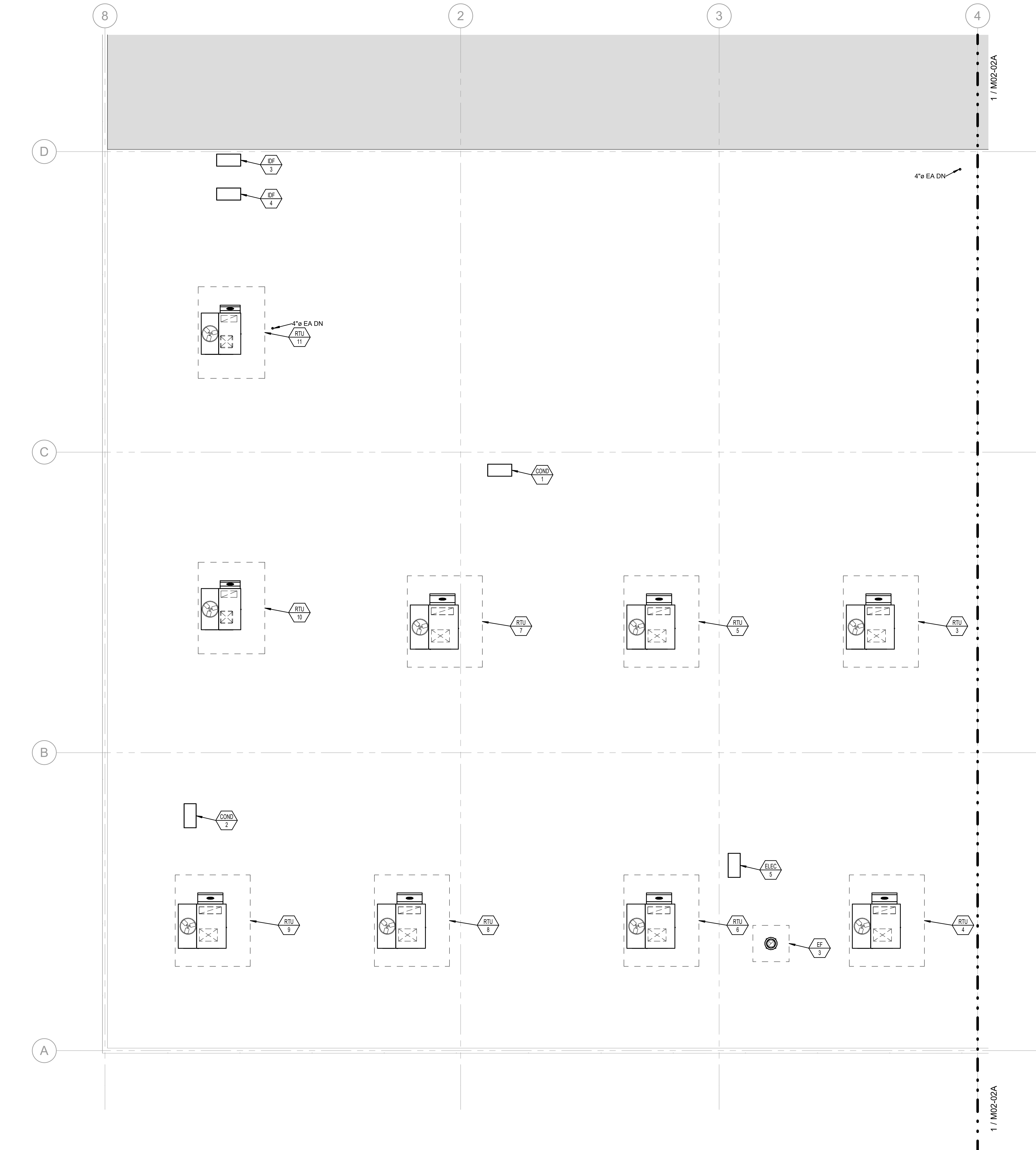
1 HVAC PLAN - ROOF - SEGMENT B SCALE: 1/8" = 1'-0"
