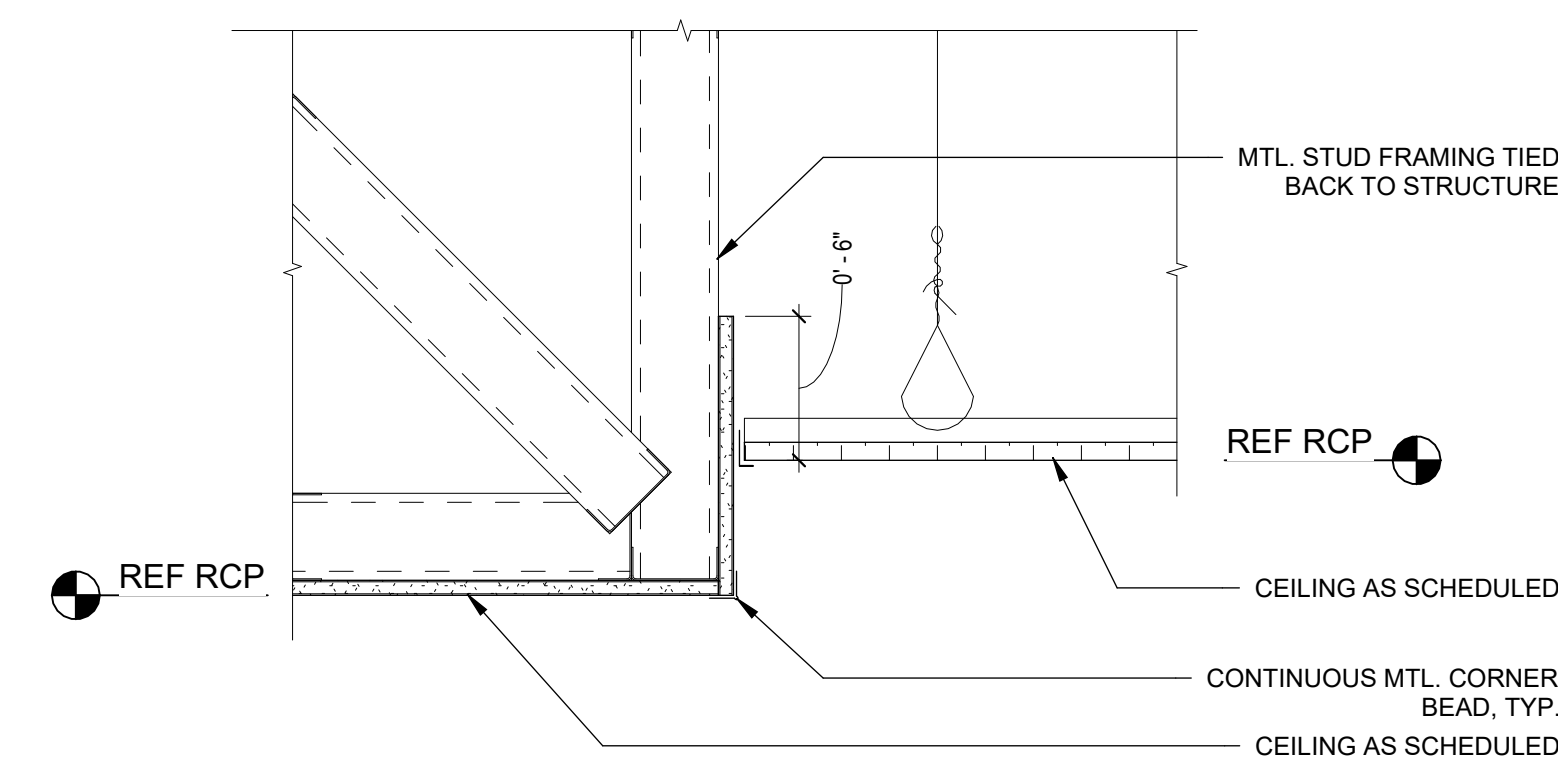
6 RCP DETAIL - GYP TO HIGHER LAY IN 1 1/2" = 1'-0"
