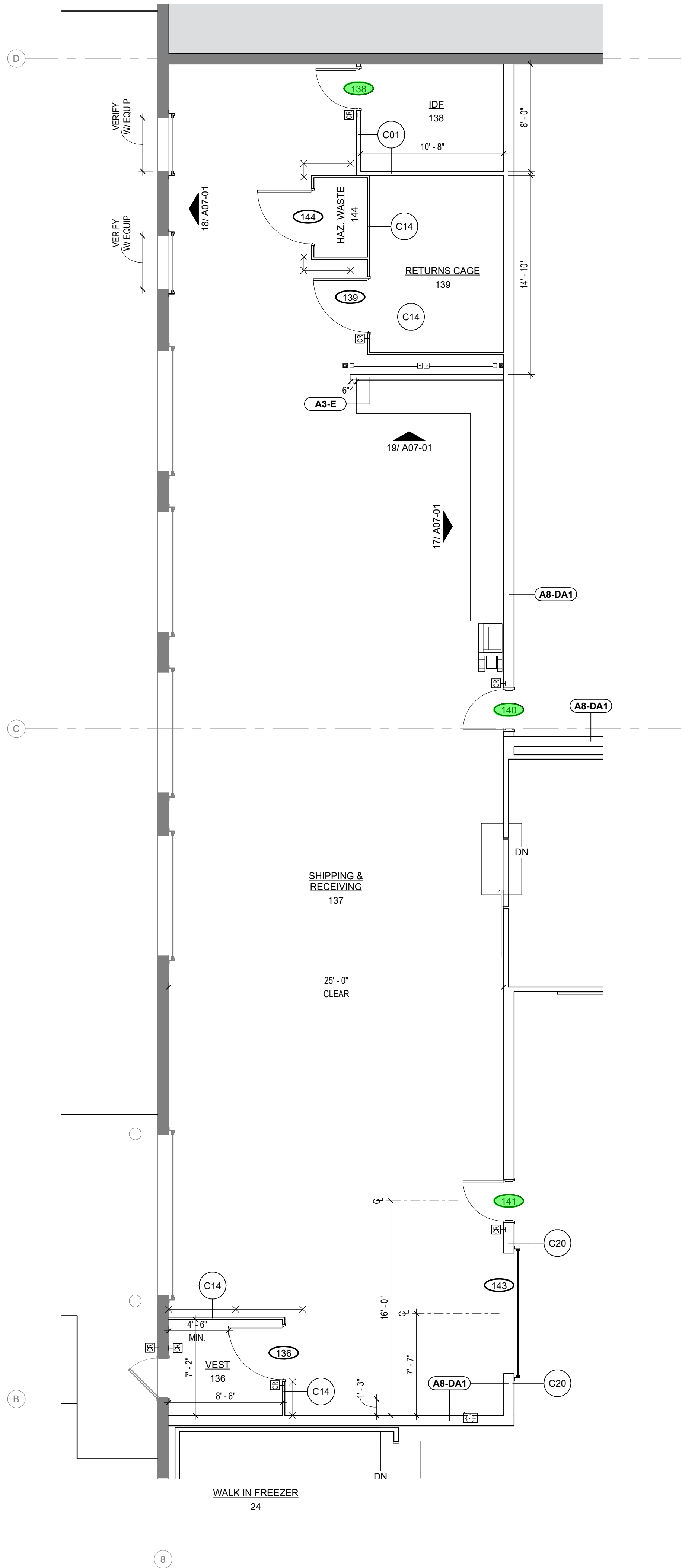
1 FLOOR PLAN - SEGMENT B 3/16" = 1'-0"
