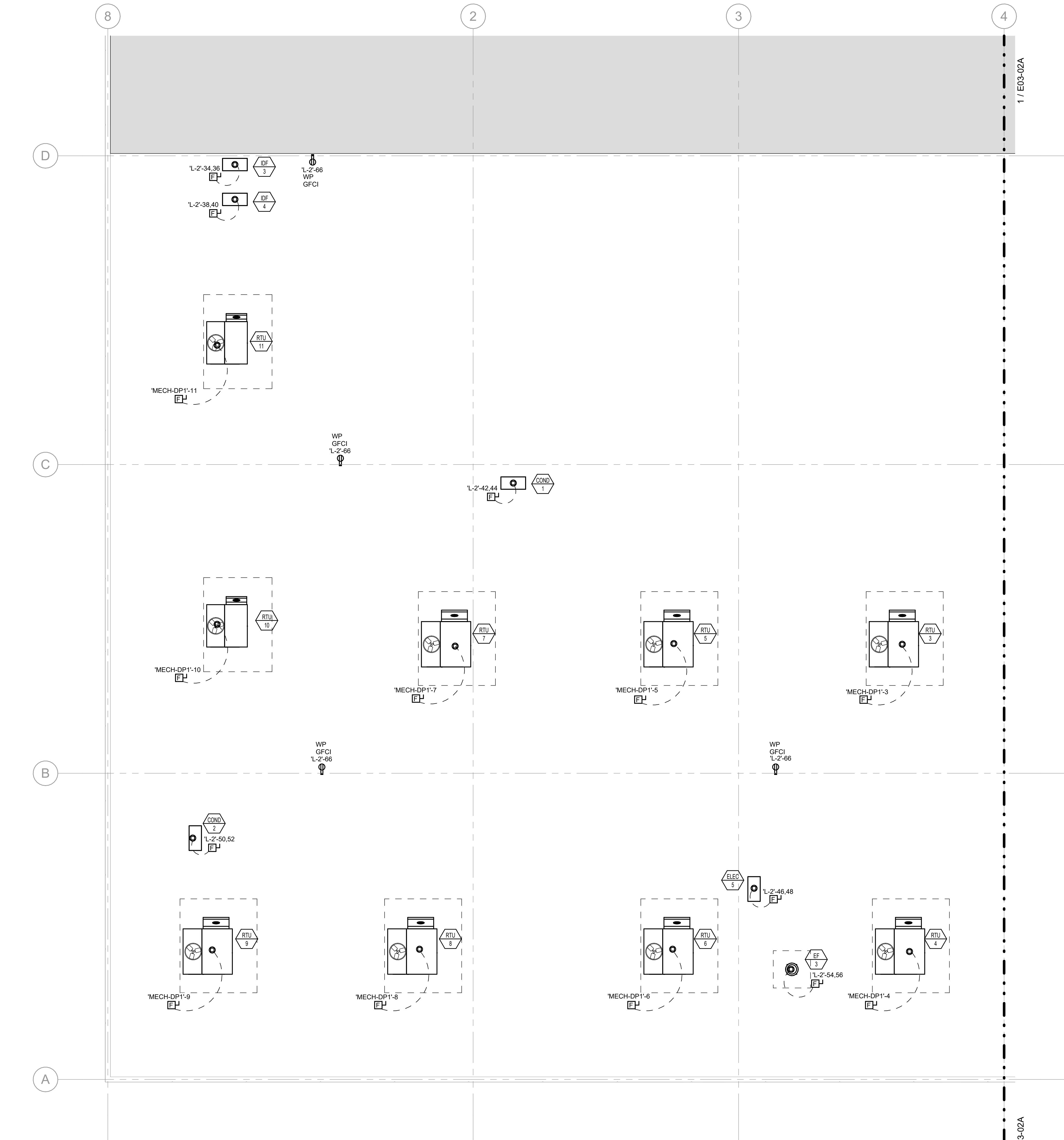
1 POWER PLAN - ROOF - SEGMENT B SCALE: 1/8" = 1'-0"
