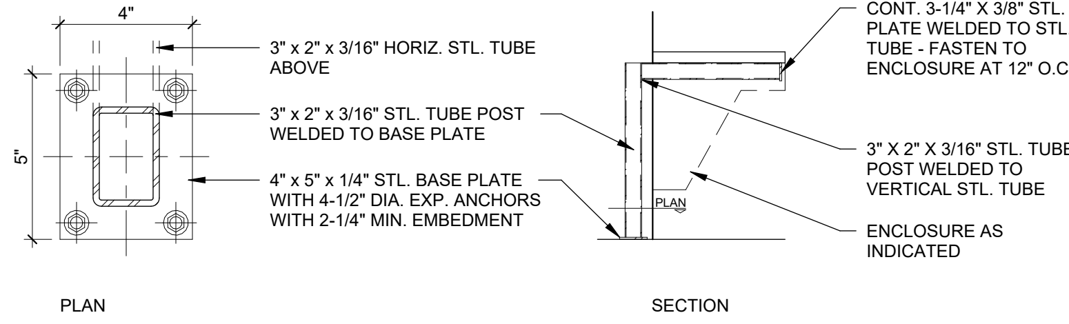
03 LAVATORY COUNTER SUPPORT - SPAN 10'-0" TO 16'-0" N.T.S.
