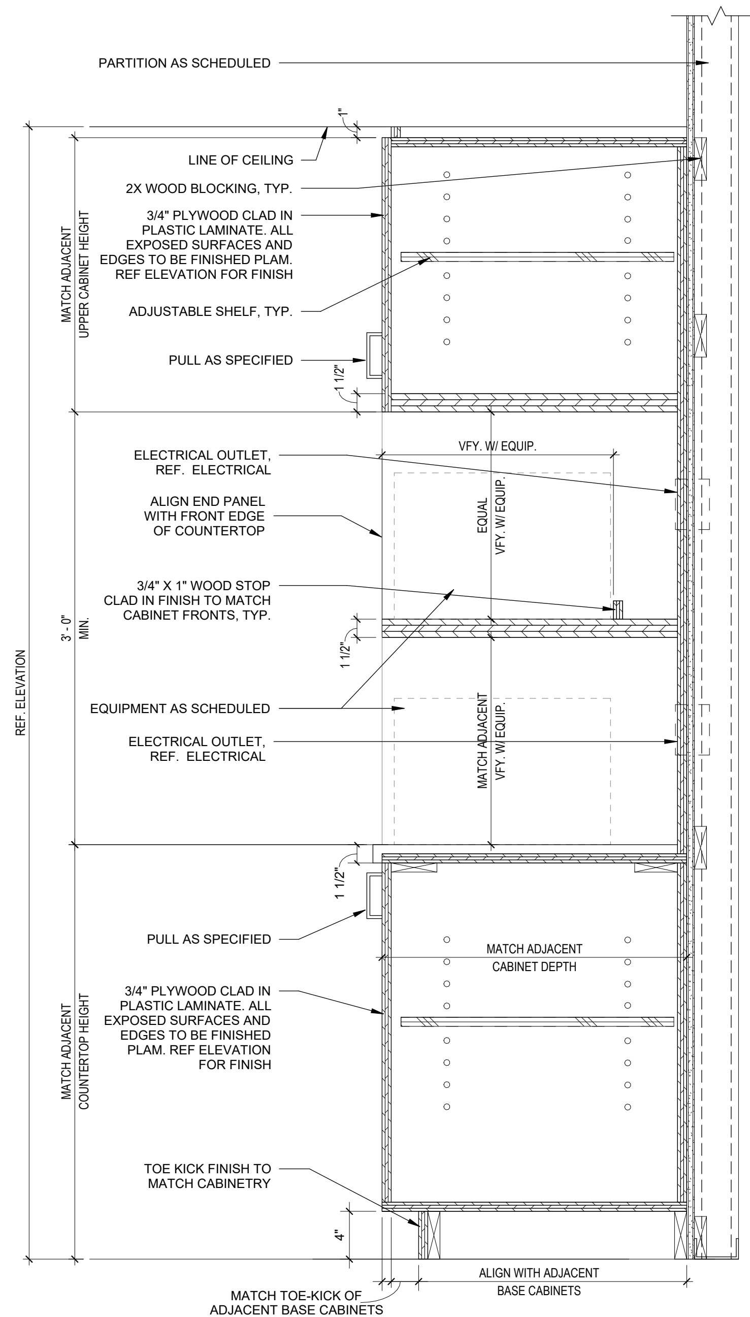
01 SECTION AT MICROWAVE CABINET 1 1/2" = 1'-0"
